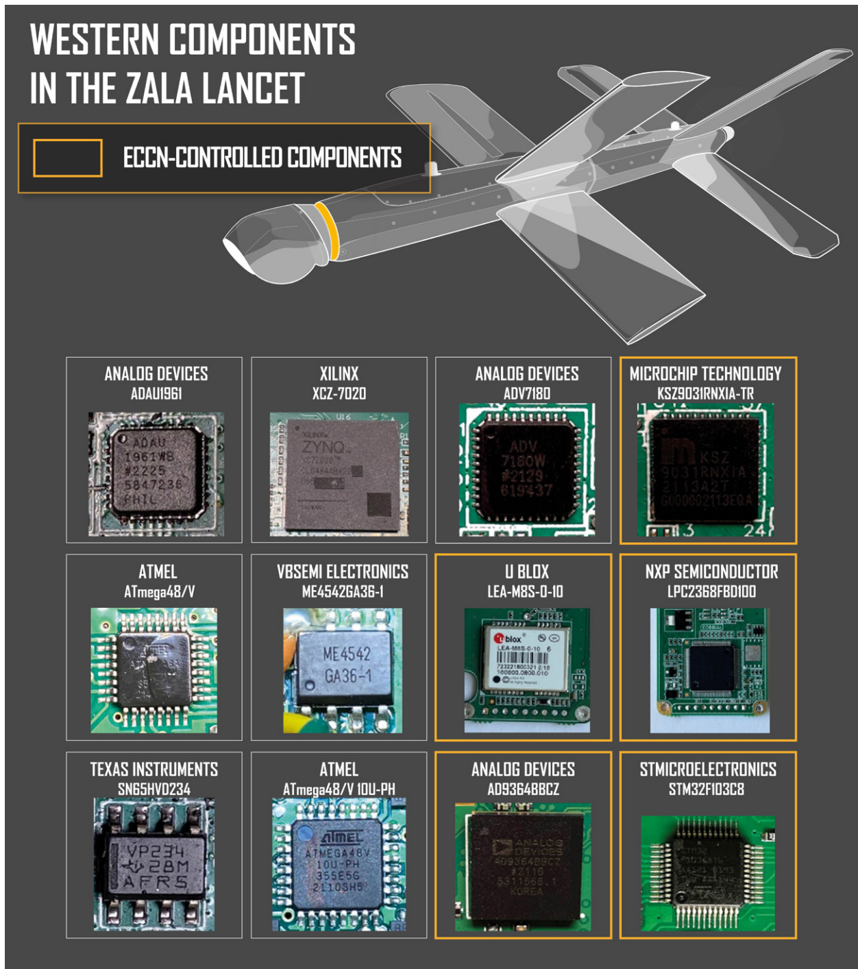
Figure 2: Western-Made Components Inside the Zala Lancet-3
